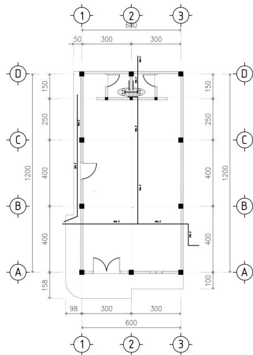
DENAH INSTALASI AIR KOTOR
